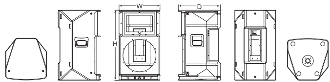
Dimension(W×H×D):439×760×454mm
