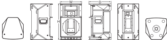
Dimension(W×H×D):356×608×372mm
