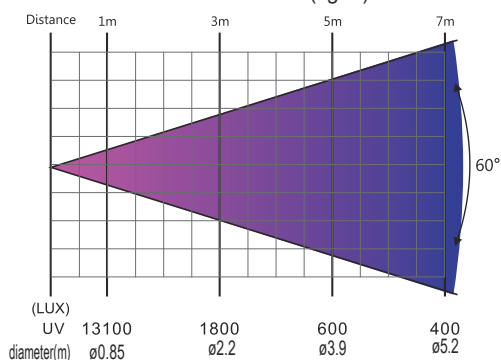
PHOTOMETRIC DIAGRAM (fig. 5)
