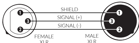
3-PIN XLR
