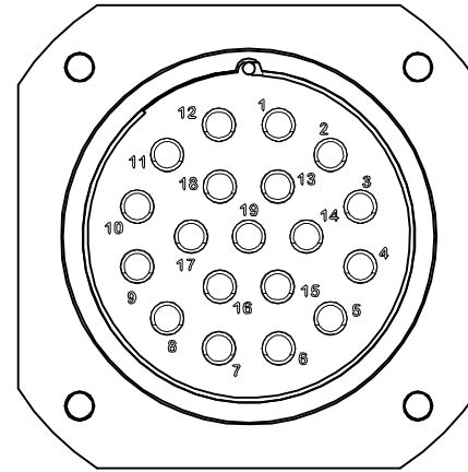
WIRING SIDE
