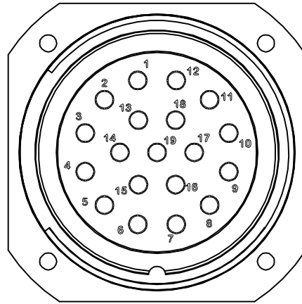
FRONT SIDE
